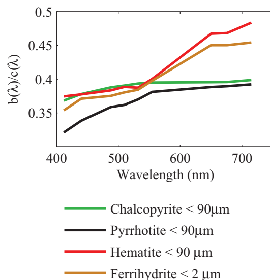
Figure 5. Spectral albedo (the fraction of beam attenuation accounted for by scattering b(\lambda) rather than absorption) of suspended, powdered iron oxide and sulfide mineral standards in water. Absorption accounts for a greater fraction of beam attenuation by sulfide minerals, than it does for oxide minerals. Measurements were collected with an ac-9 in the laboratory, and data were processed and corrected similarly to field data described in the text. Particle maximum diameters are given in the legend.
